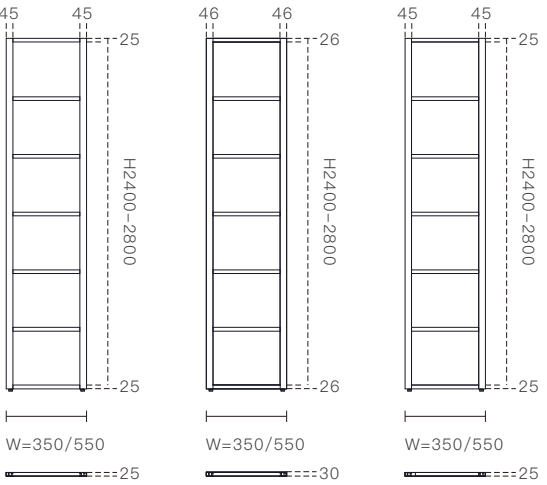
艾瑞-无玻璃铝栅 H=2400-2800mm W=350/550mm D=25mm 艾瑞-通体玻璃铝栅 H=2400-2800mm W=350/550mm D=30mm 艾瑞-内嵌木板铝栅 H=2400-2800mm W=350/550mm D=25mm
